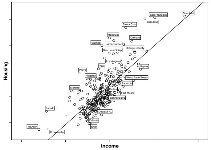
Fig 3: Scatter-graphs
