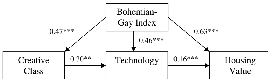
Fig. 6: Path models for housing, technology and the Bohemian-Gay Index
